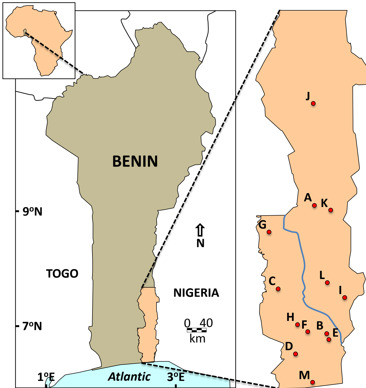
Figure 1. Location of the study area in the Ouémé-Plateau in southeastern Benin. Study districts include: A. Adja-Ouèrè, B. Adjarra, C. Adjohoun, D. Aguégoués, E. Akpro-Missérété, F. Avrankou, G. Bonou, H. Dangbo, I. Ifangni, J. Kétou, K. Pobè, L. Sakété, and M. Sèmè-Kpodji.
